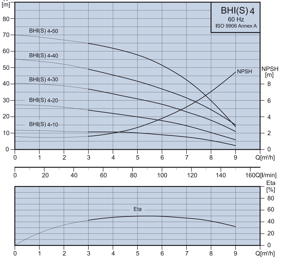
Performance curves 60 Hz
